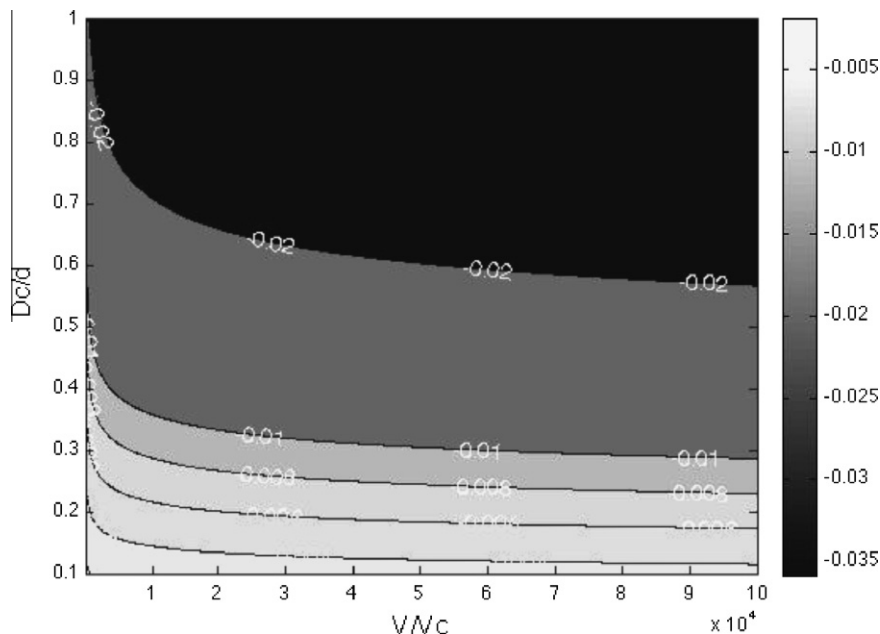
Fig. 5. Contours of v_e for the parameter space of critical slip distance (ordinate) versus critical sliding velocity (abscissa) for a brittle friction loss mechanism.
