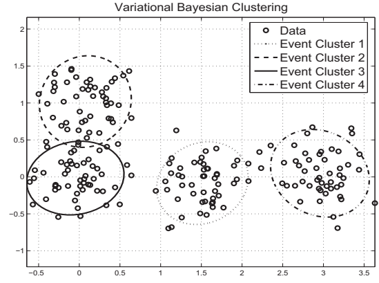
Fig. 5. Clustering of event prototypes using the VBGM approach.
