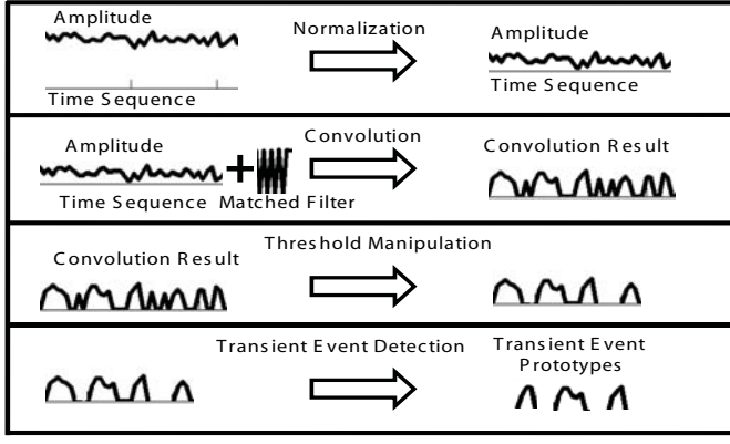
Fig. 3. The procedure of event prototype generation.
