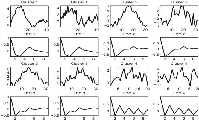
Fig. 4. Compressive linear predictive coding of signal events.
